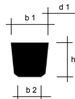
Form F LKD Deckel / cover
